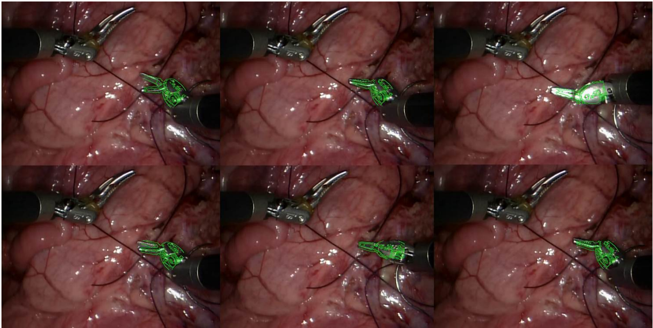
Fig. 8 Sample output frames from running the tool detector on an in-vivo video sequence. Several different poses are shown as well as an example with high specularity (top-right). The green overlay is produced by drawing only the edges of the best-matching virtually-rendered template, to assist in seeing the quality of the result. These results are produced from the pyramid-search method, described in section 3.2.1.
