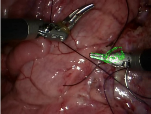
Fig. 7 A failure case is defined as a detection that occurs on the correct tool tip with a visibly-wrong joint configuration.
