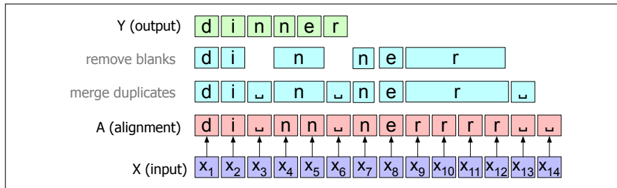
Figure 26.8 The CTC collapsing function B , showing the space blank character \sqcup ; repeated (consecutive) characters in an alignment A are removed to form the output Y .
