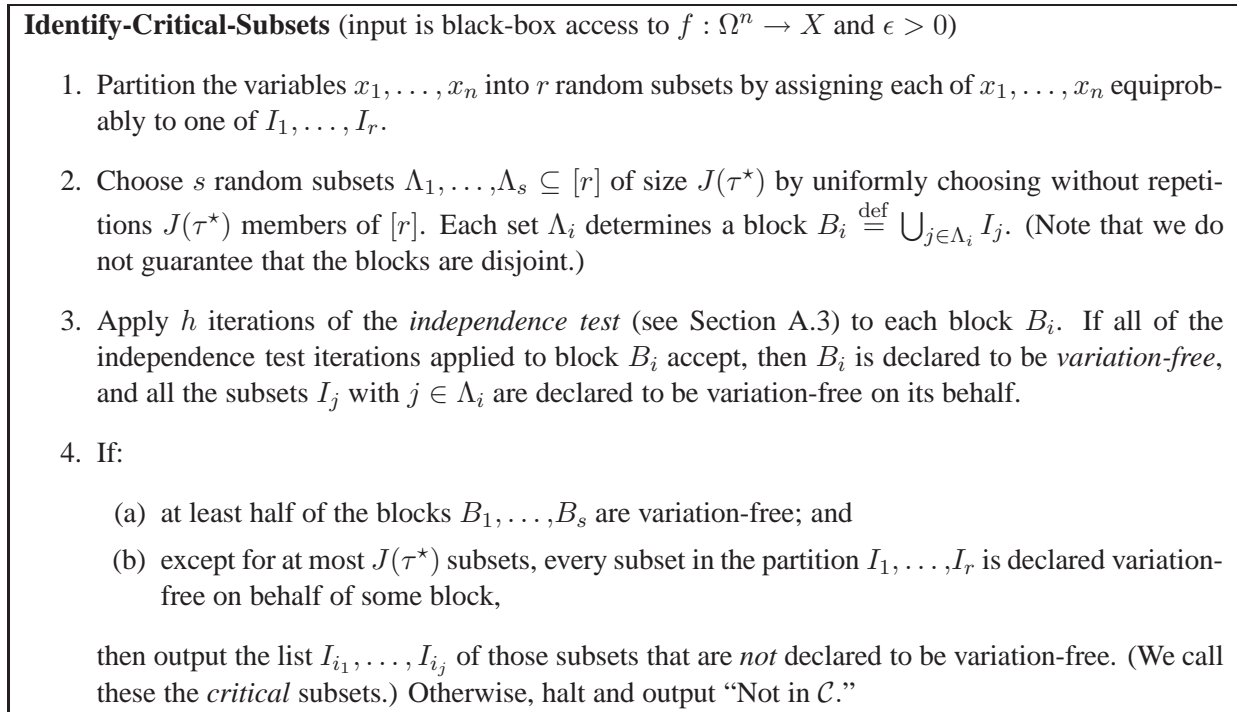
Figure 4: The subroutine Identify-Critical-Subsets .
