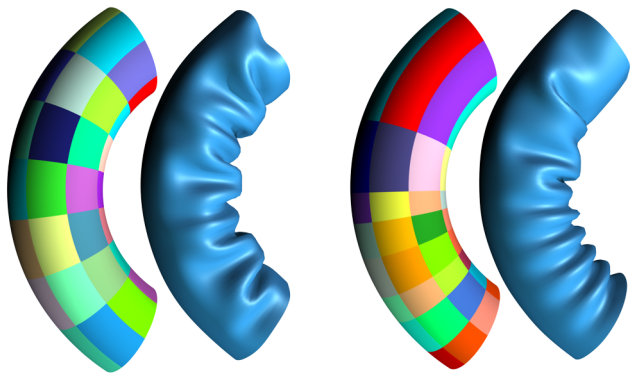
Figure 5: Spatially varying test functions . Buckling of the tracked surface is directly linked to the distribution of test functions over the mesh. A homogeneous distribution ( left ) results in uniform wrinkling of the surface, whereas a heterogeneous distribution ( right ) causes larger folds to form in coarser regions and smaller wrinkles to form in finer-support regions.
