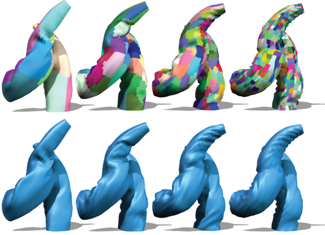
Figure 6: Constraint resolution . Increasing the number of partitions (left-to-right: 16, 64, 256, 1024) narrows the support of the test functions, forcing closer tracking and finer wrinkles.
