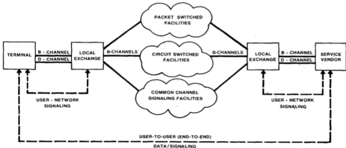
Fig. 7. The three-cloud network.
